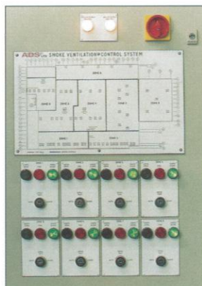
WELLSTREAM NORTH SEA 1 master 8 zone smoke ventilation control panel
